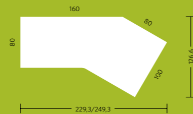
Multi-Arbeitstisch Multi-worktable
